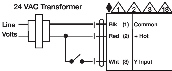
24 VAC Transformer
