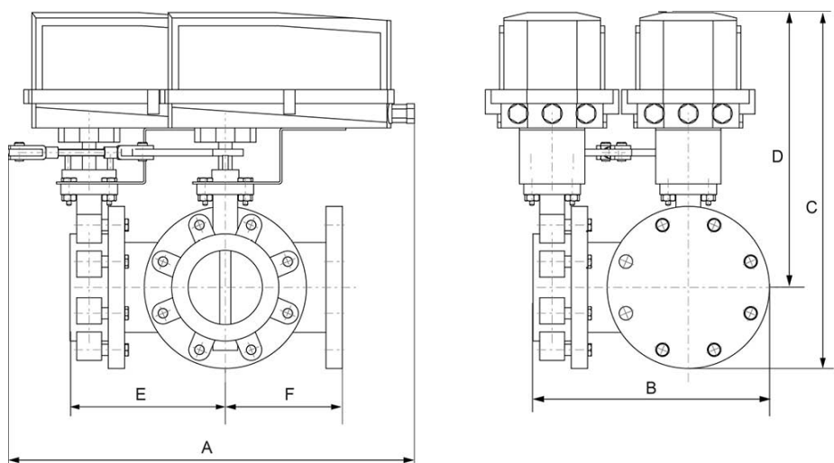
Valve with 2*GMCX24-3-T-X1 N4 Actuator
